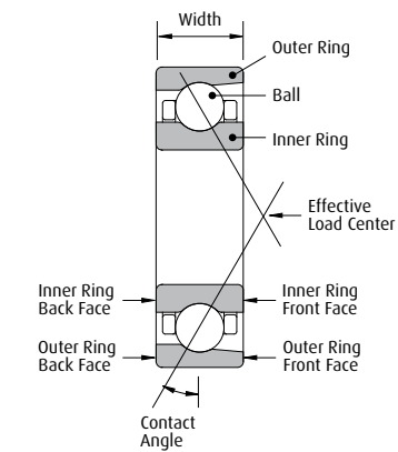
Single Row Angular Contact Ball Bearing
