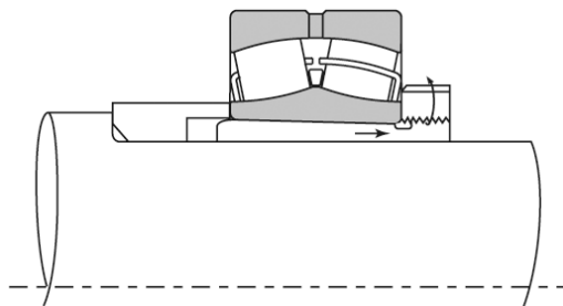
Mounting w/Adapter
